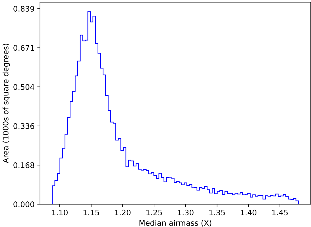
too_elab_r64_d3_giz_v3.4_10yrs WFD z band: Median airmass
