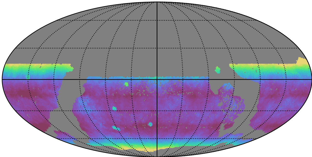
too_elab_r64_d3_giz_v3.4_10yrs WFD y band: Median airmass
