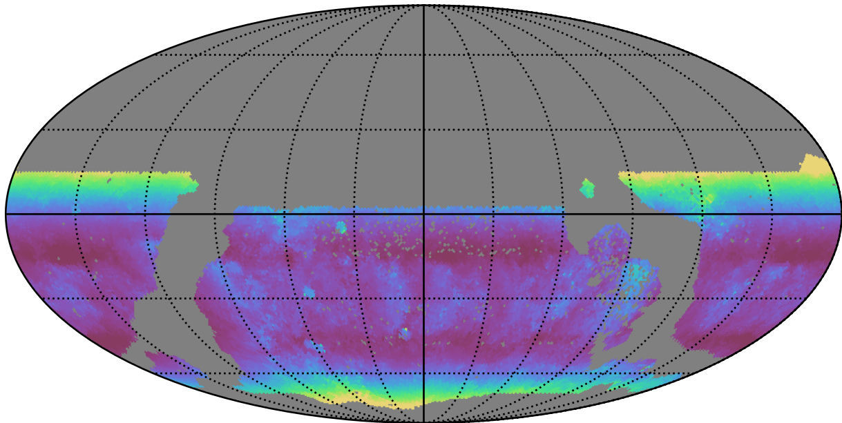
too_elab_r64_d3_giz_v3.4_10yrs WFD u band: Median airmass
