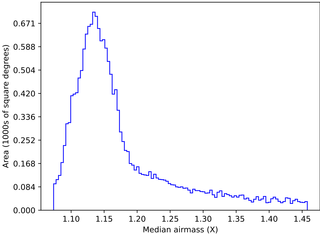
too_elab_r64_d3_giz_v3.4_10yrs WFD r band: Median airmass
