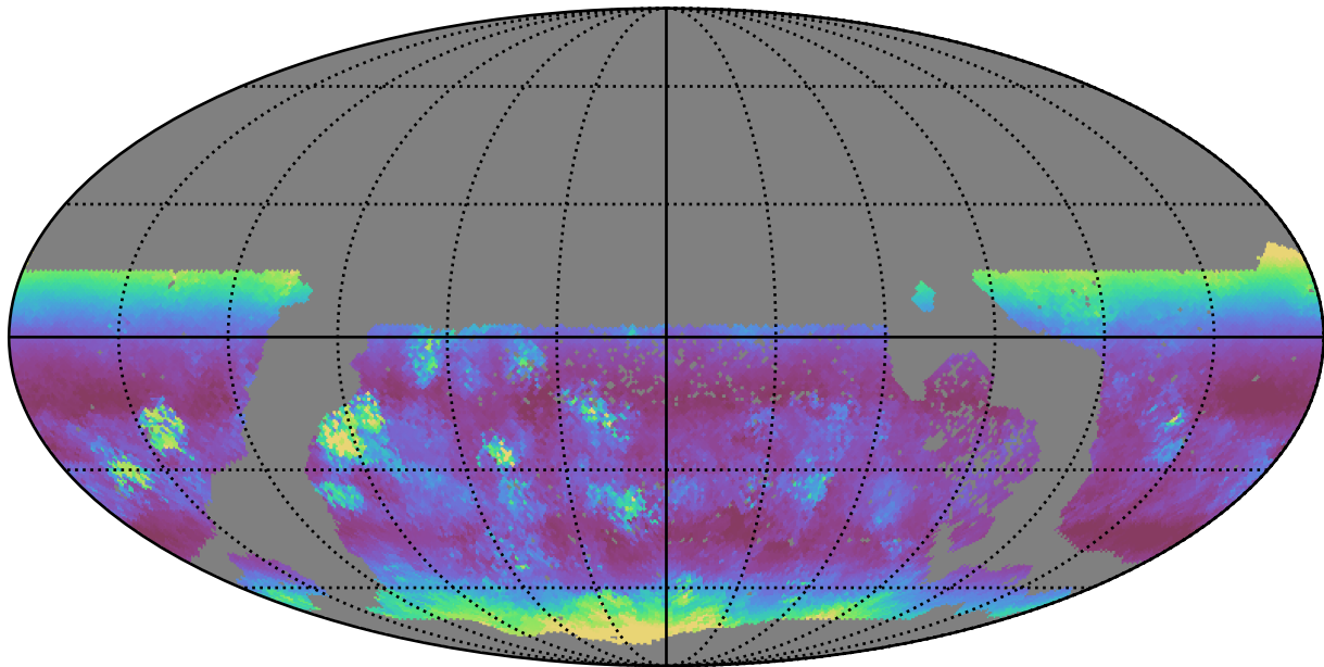
too_elab_r64_d3_giz_v3.4_10yrs WFD g band: Median airmass
