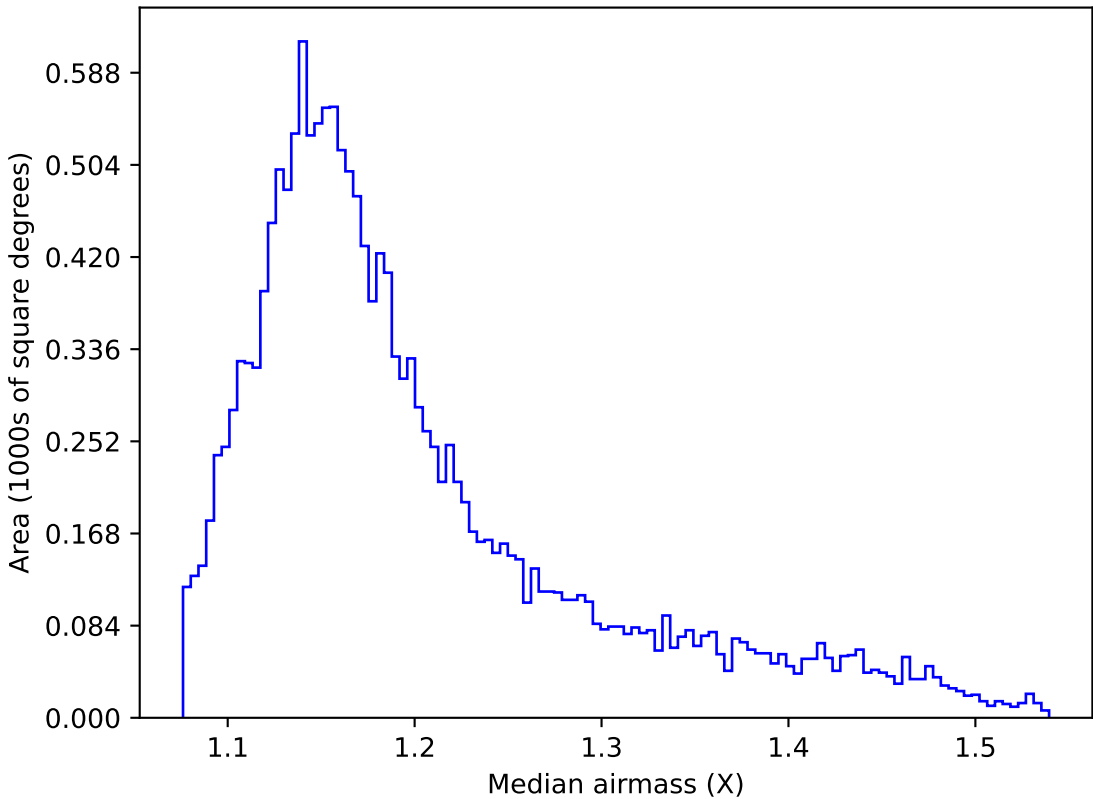
too_elab_r64_d3_giz_v3.4_10yrs WFD g band: Median airmass
