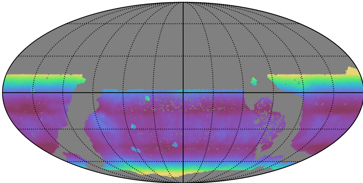
too_elab_r64_d3_giz_v3.4_10yrs WFD all bands: Median airmass
