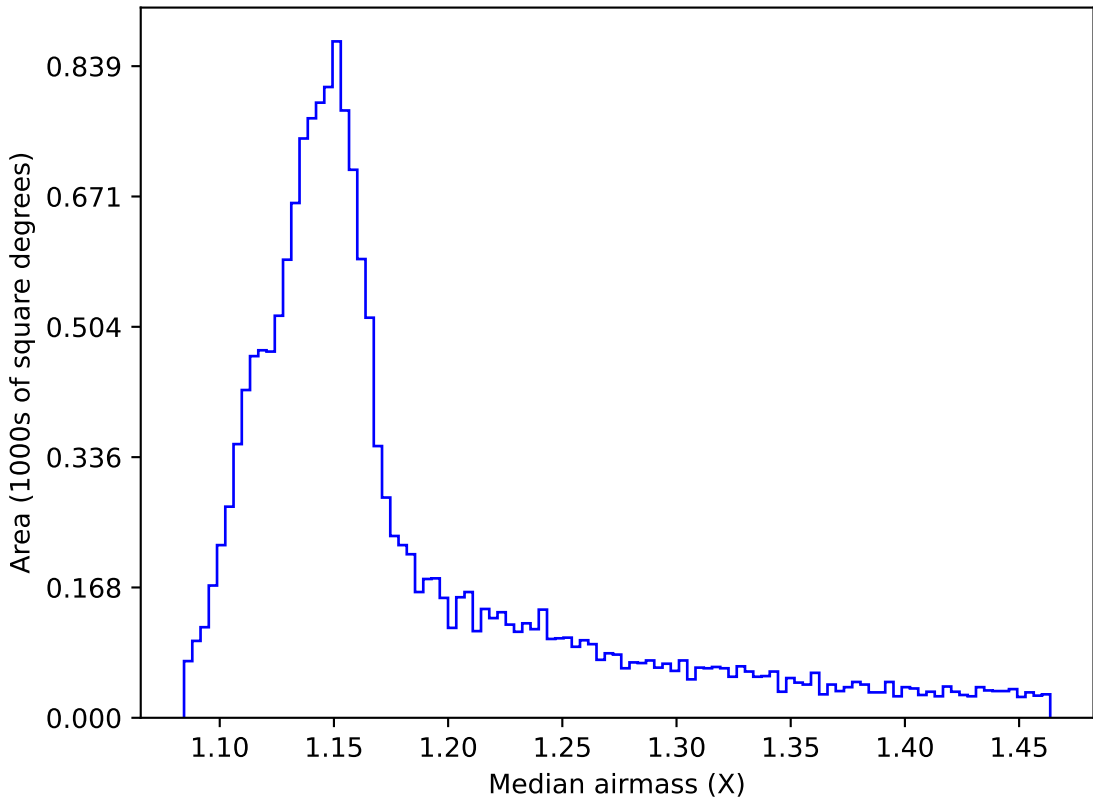
too_elab_r64_d3_giz_v3.4_10yrs WFD all bands: Median airmass
