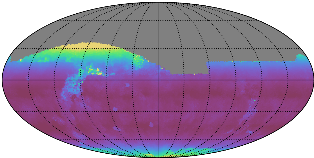
too_elab_r64_d3_giz_v3.4_10yrs All sky z band: Median airmass
