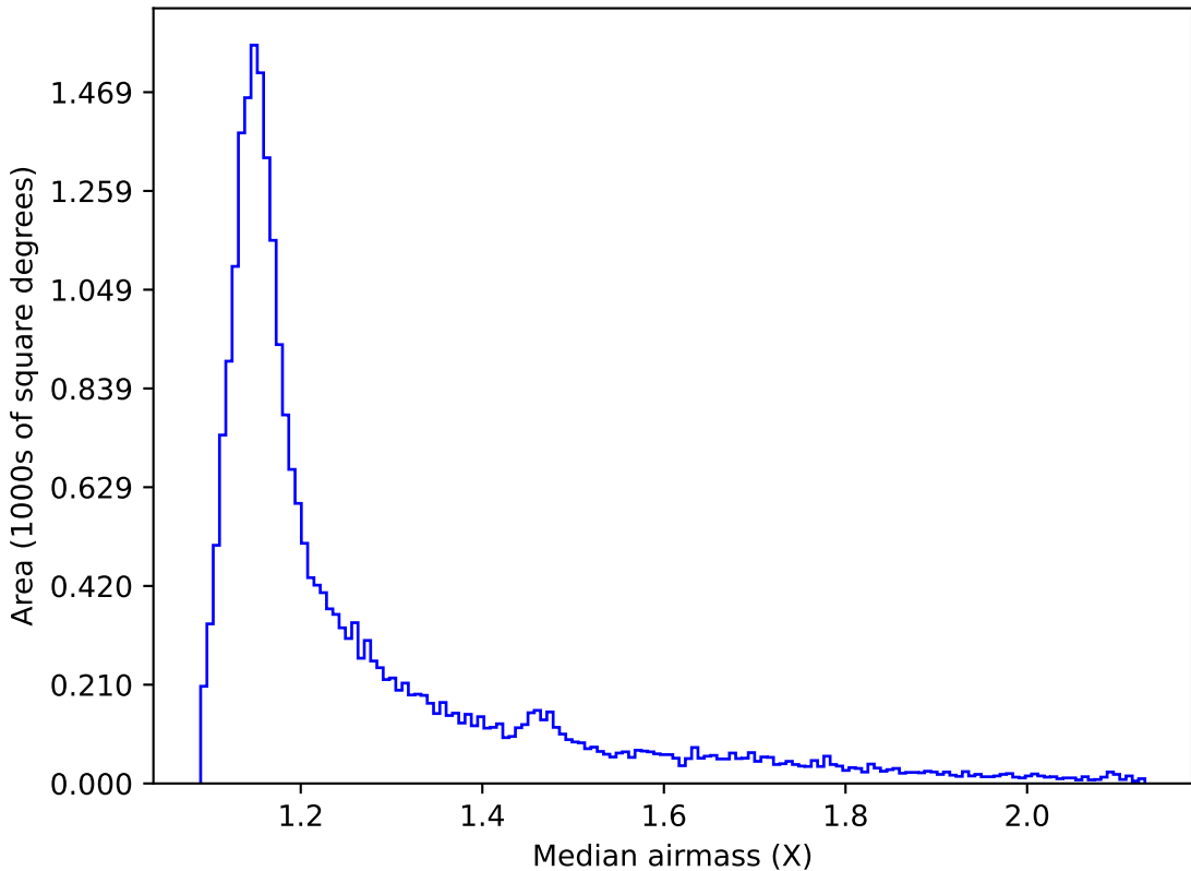
too_elab_r64_d3_giz_v3.4_10yrs All sky z band: Median airmass
