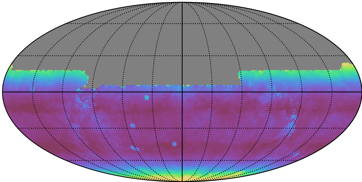
too_elab_r64_d3_giz_v3.4_10yrs All sky y band: Median airmass
