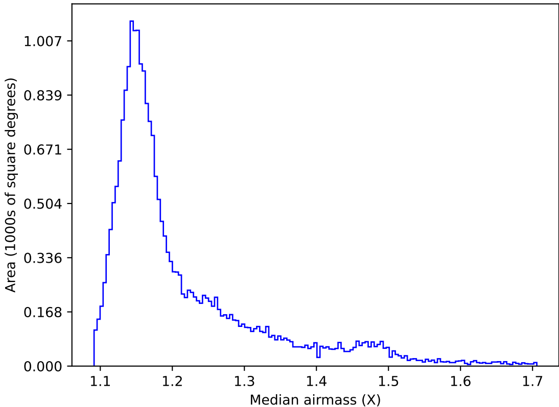
too_elab_r64_d3_giz_v3.4_10yrs All sky y band: Median airmass
