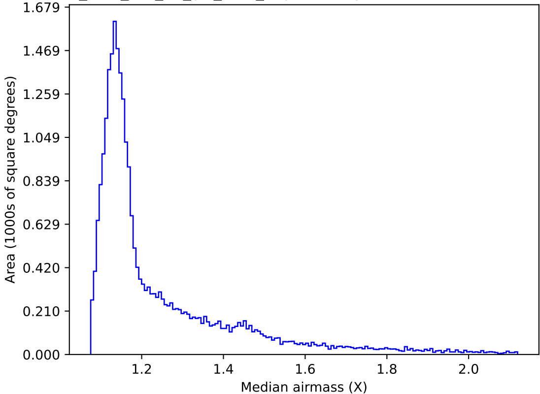
too_elab_r64_d3_giz_v3.4_10yrs All sky r band: Median airmass
