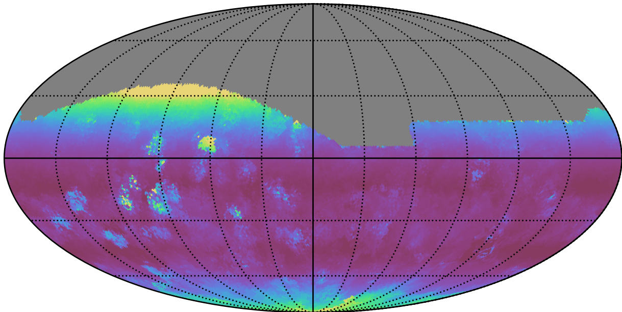
too_elab_r64_d3_giz_v3.4_10yrs All sky g band: Median airmass
