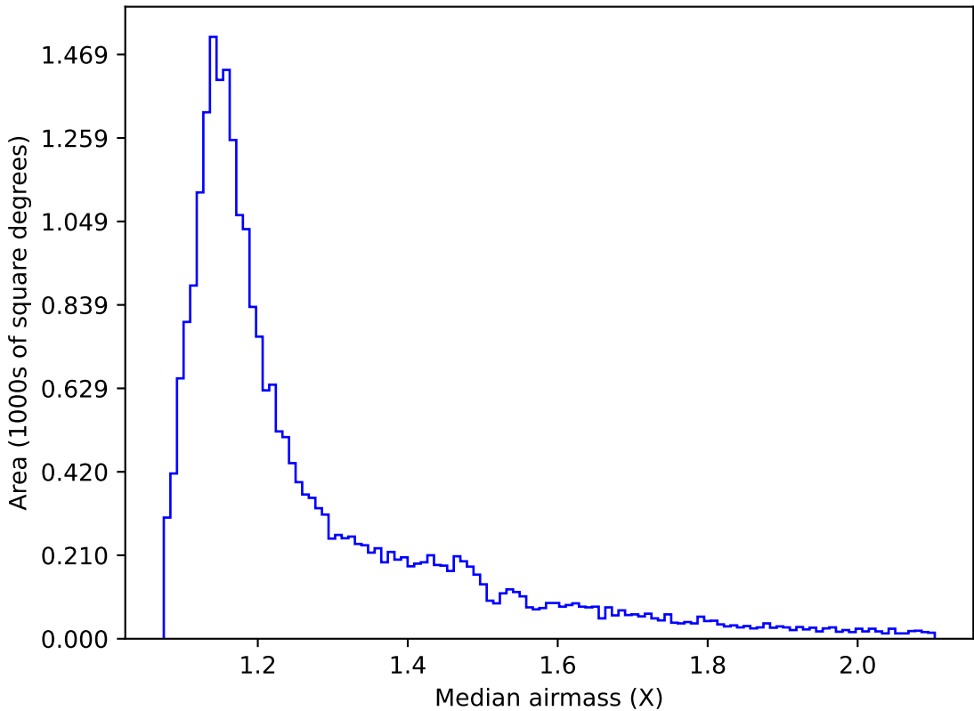
too_elab_r64_d3_giz_v3.4_10yrs All sky g band: Median airmass
