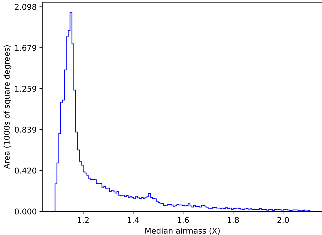
too_elab_r64_d3_giz_v3.4_10yrs All sky all bands: Median airmass
