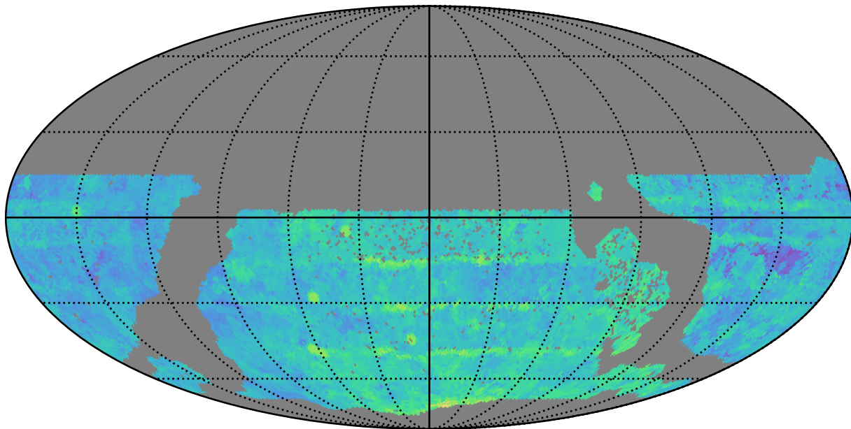
too_elab_r64_d3_giz_v3.4_10yrs WFD z band: Median Season Length
