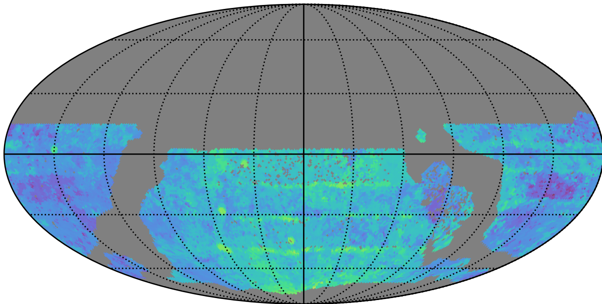
too_elab_r64_d3_giz_v3.4_10yrs WFD y band: Median Season Length
