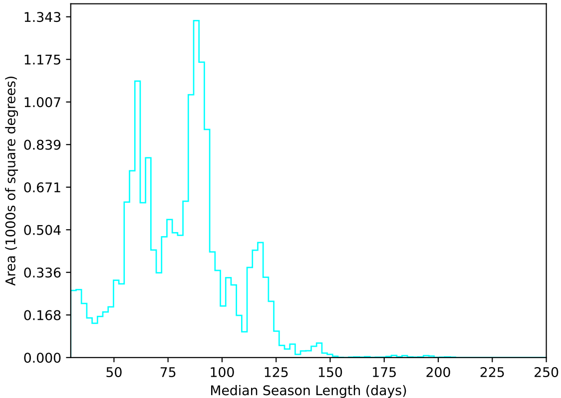
too_elab_r64_d3_giz_v3.4_10yrs WFD u band: Median Season Length
