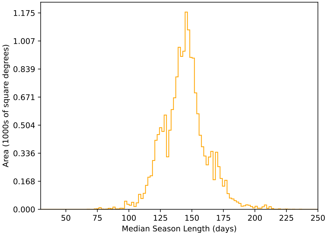
too_elab_r64_d3_giz_v3.4_10yrs WFD r band: Median Season Length
