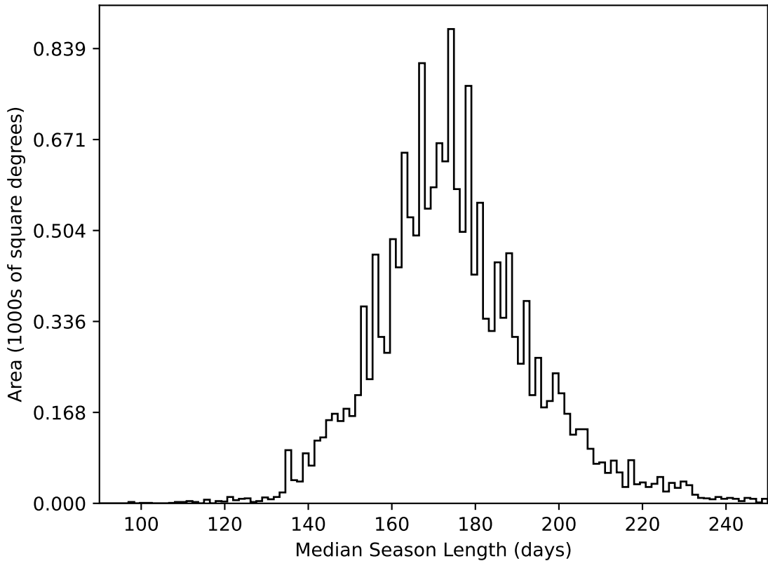
too_elab_r64_d3_giz_v3.4_10yrs WFD all bands: Median Season Length
