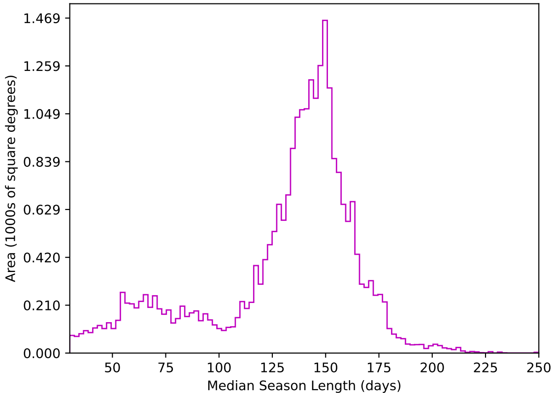
too_elab_r64_d3_giz_v3.4_10yrs All sky z band: Median Season Length
