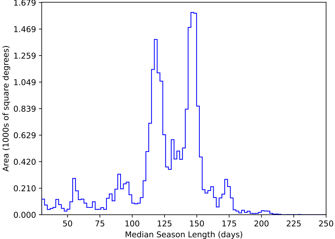
too_elab_r64_d3_giz_v3.4_10yrs All sky y band: Median Season Length
