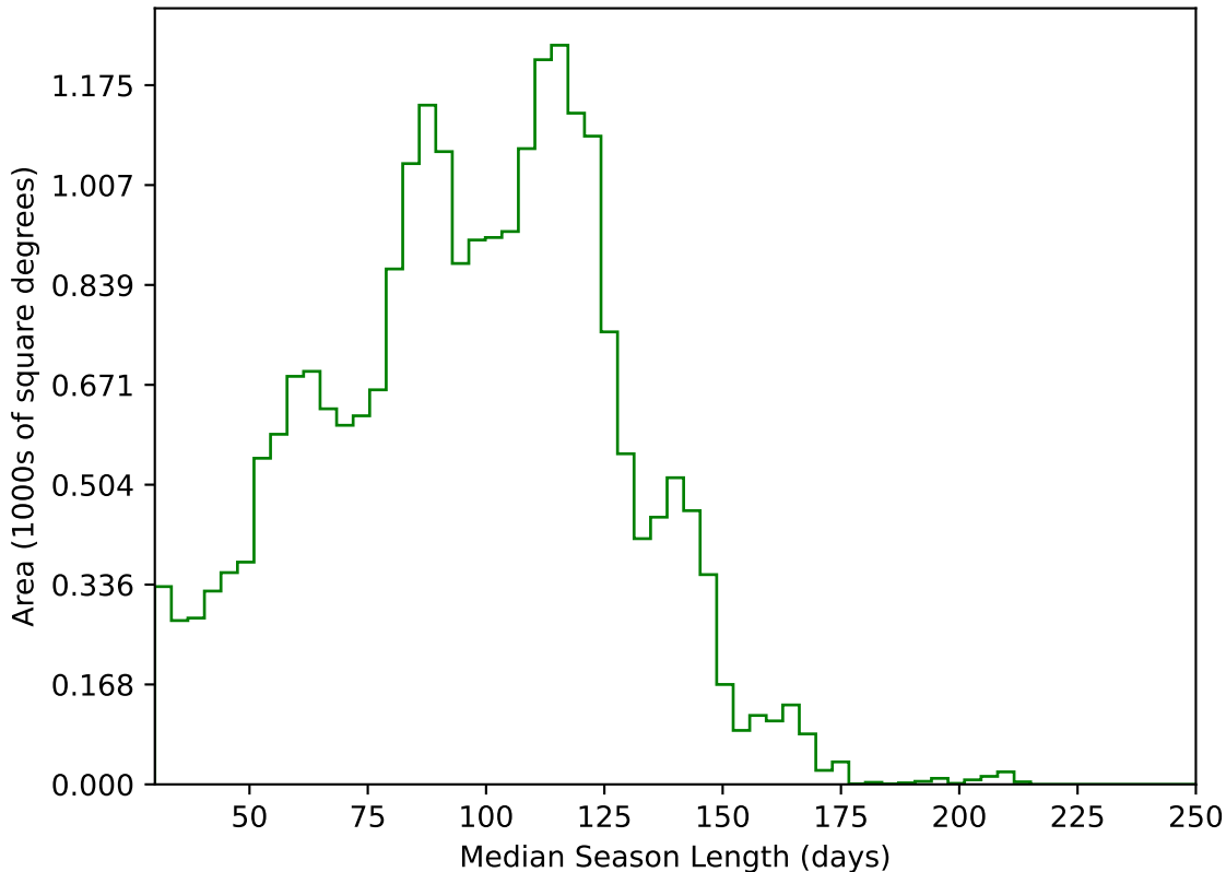
too_elab_r64_d3_giz_v3.4_10yrs All sky g band: Median Season Length
