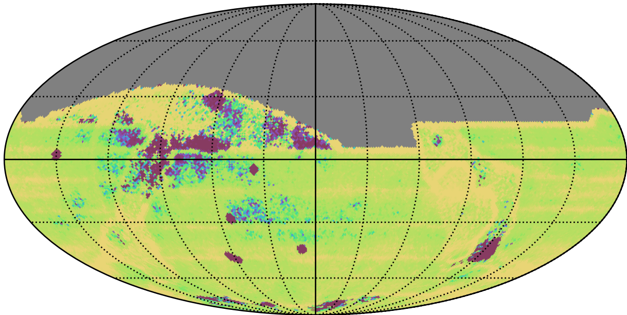
too_elab_r64_d3_giz_v3.4_10yrs All sky: Median Intra-Night Gap
