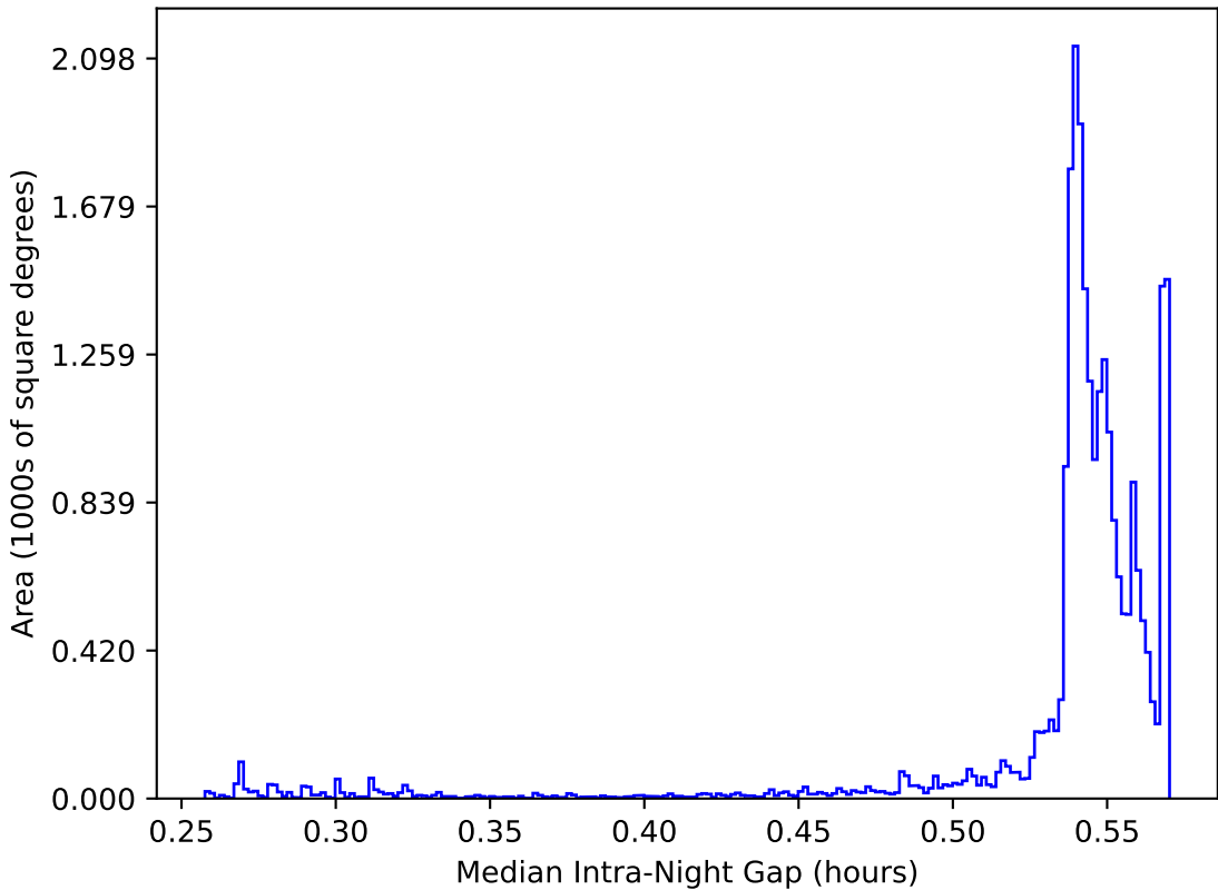
too_elab_r64_d3_giz_v3.4_10yrs All sky: Median Intra-Night Gap
