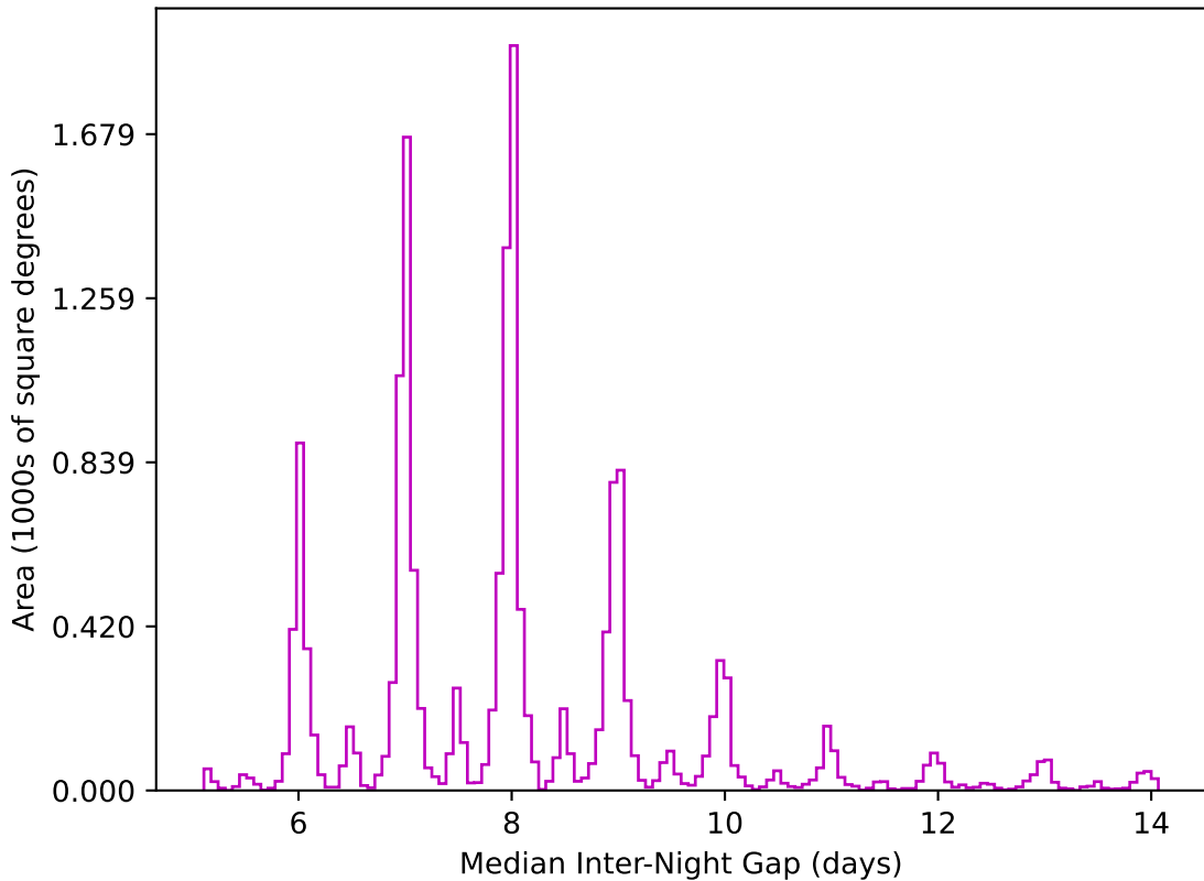
too_elab_r64_d3_giz_v3.4_10yrs WFD z band: Median Inter-Night Gap
