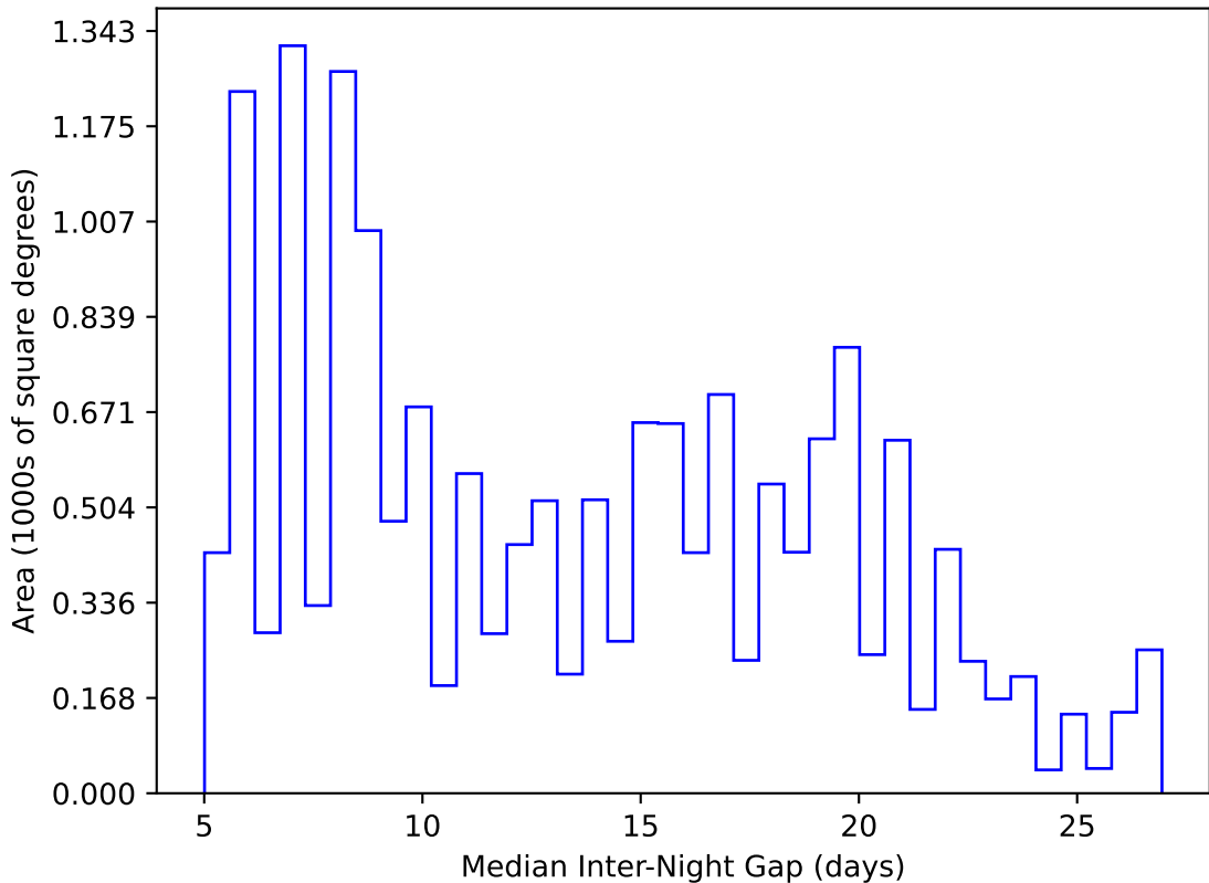
too_elab_r64_d3_giz_v3.4_10yrs WFD y band: Median Inter-Night Gap
