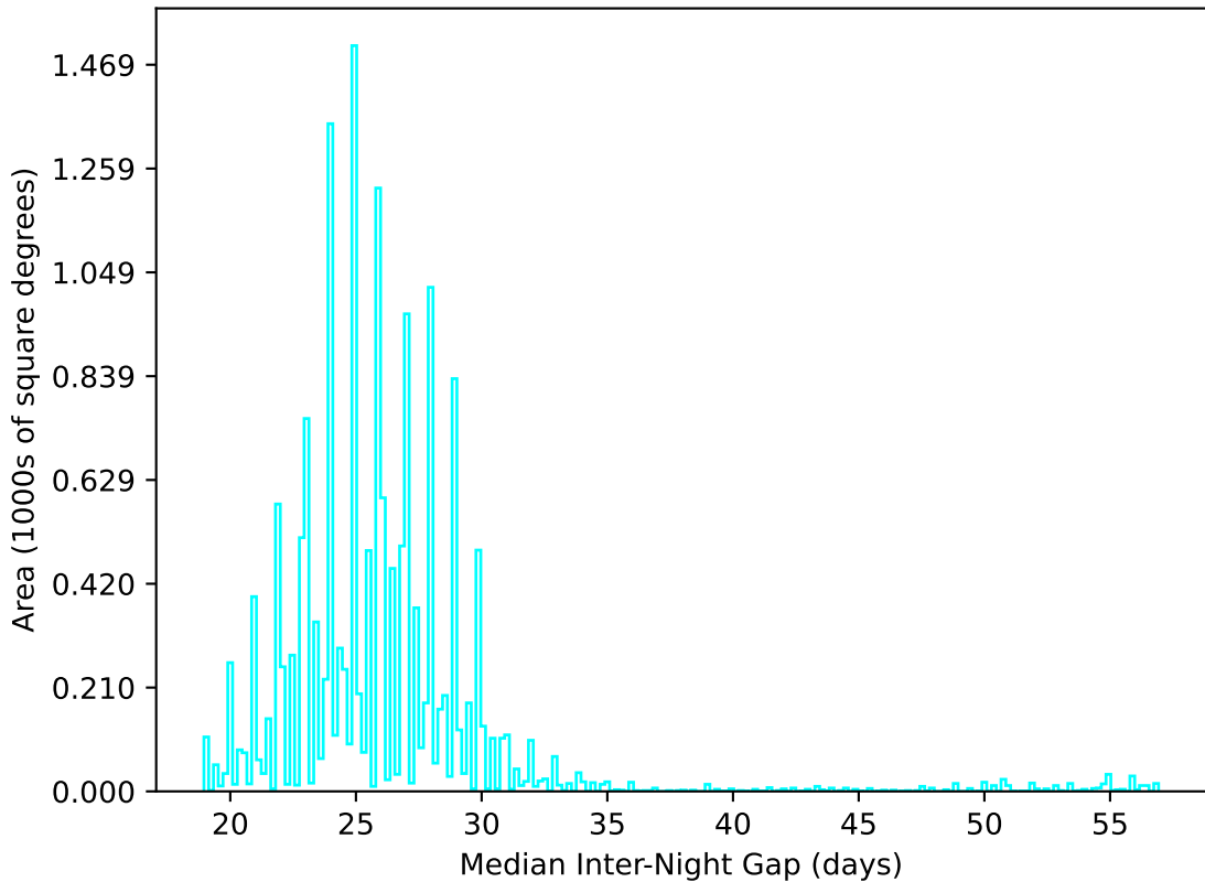
too_elab_r64_d3_giz_v3.4_10yrs WFD u band: Median Inter-Night Gap
