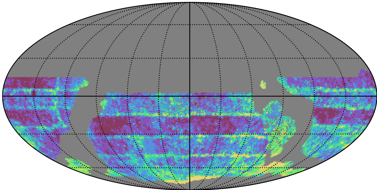
too_elab_r64_d3_giz_v3.4_10yrs WFD r band: Median Inter-Night Gap
