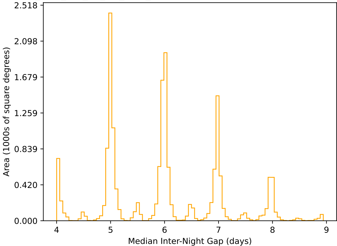
too_elab_r64_d3_giz_v3.4_10yrs WFD r band: Median Inter-Night Gap
