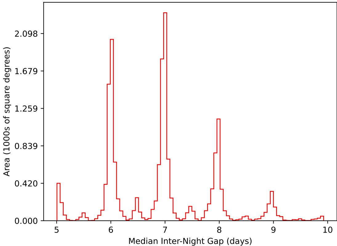
too_elab_r64_d3_giz_v3.4_10yrs WFD i band: Median Inter-Night Gap
