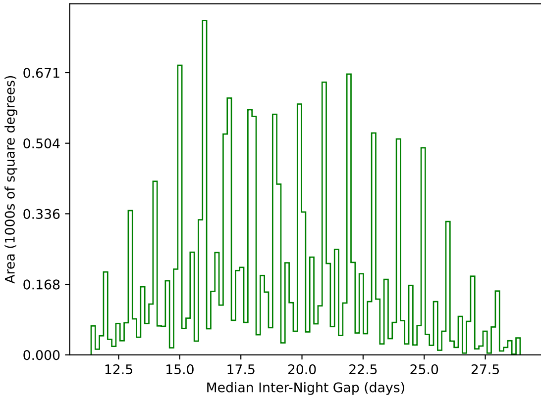
too_elab_r64_d3_giz_v3.4_10yrs WFD g band: Median Inter-Night Gap
