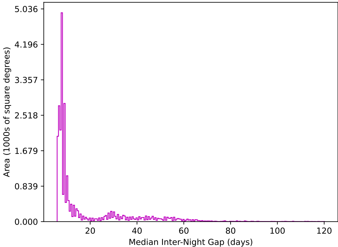
too_elab_r64_d3_giz_v3.4_10yrs All sky z band: Median Inter-Night Gap
