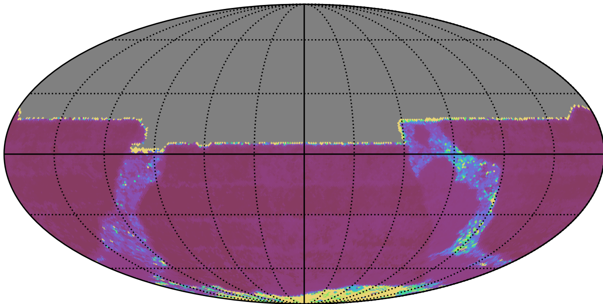
too_elab_r64_d3_giz_v3.4_10yrs All sky y band: Median Inter-Night Gap
