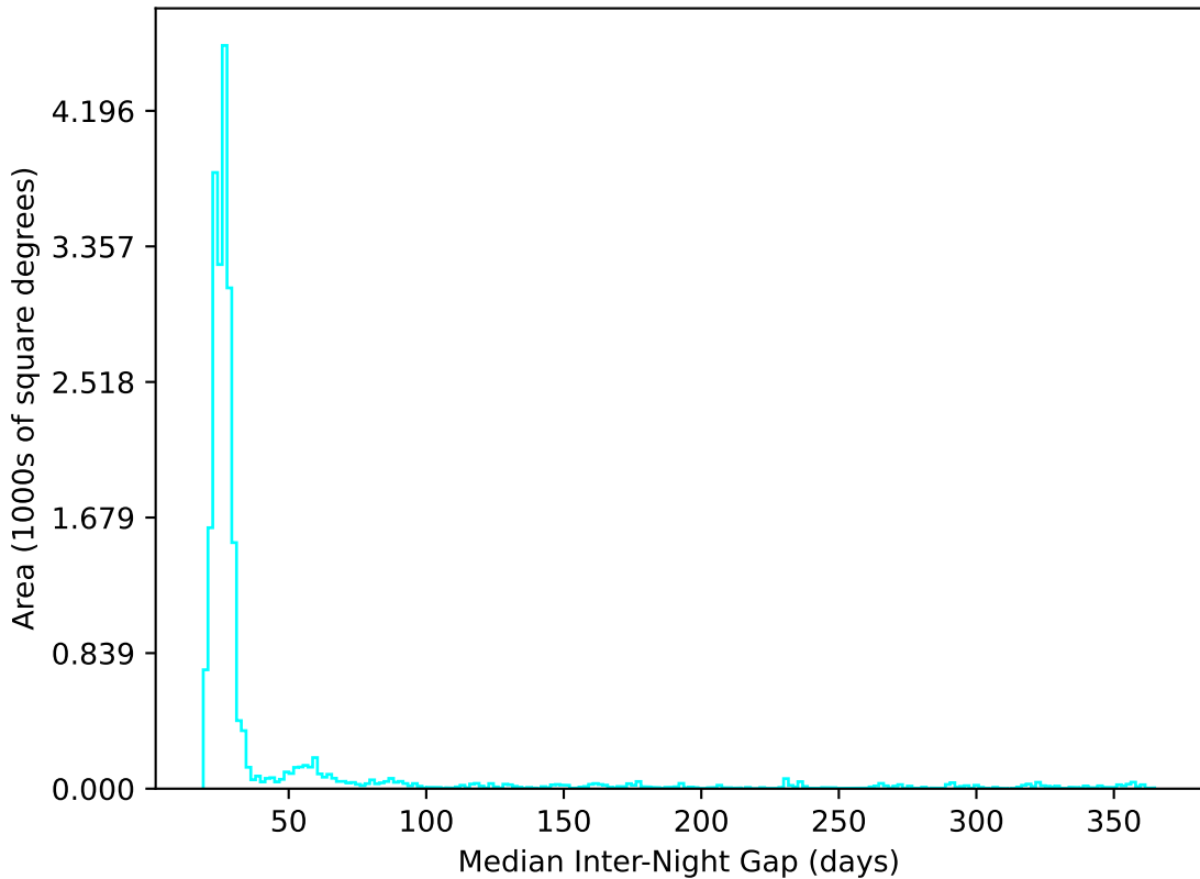
too_elab_r64_d3_giz_v3.4_10yrs All sky u band: Median Inter-Night Gap
