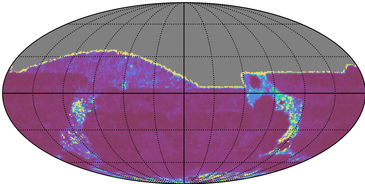
too_elab_r64_d3_giz_v3.4_10yrs All sky g band: Median Inter-Night Gap
