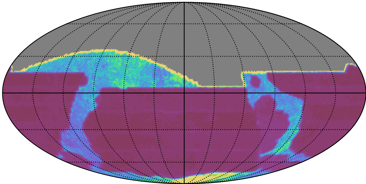
too_elab_r64_d3_giz_v3.4_10yrs All sky all bands: Median Inter-Night Gap
