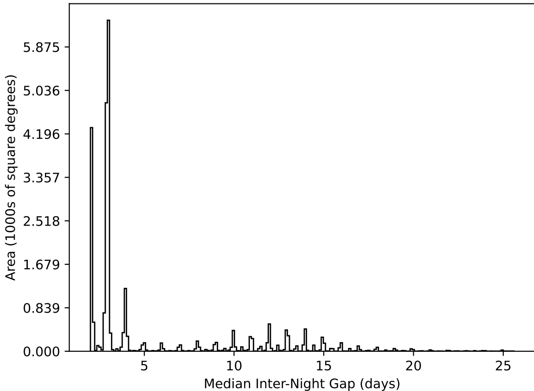
too_elab_r64_d3_giz_v3.4_10yrs All sky all bands: Median Inter-Night Gap
