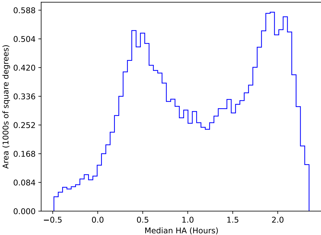
too_elab_r64_d3_giz_v3.4_10yrs WFD z band: Median HA
