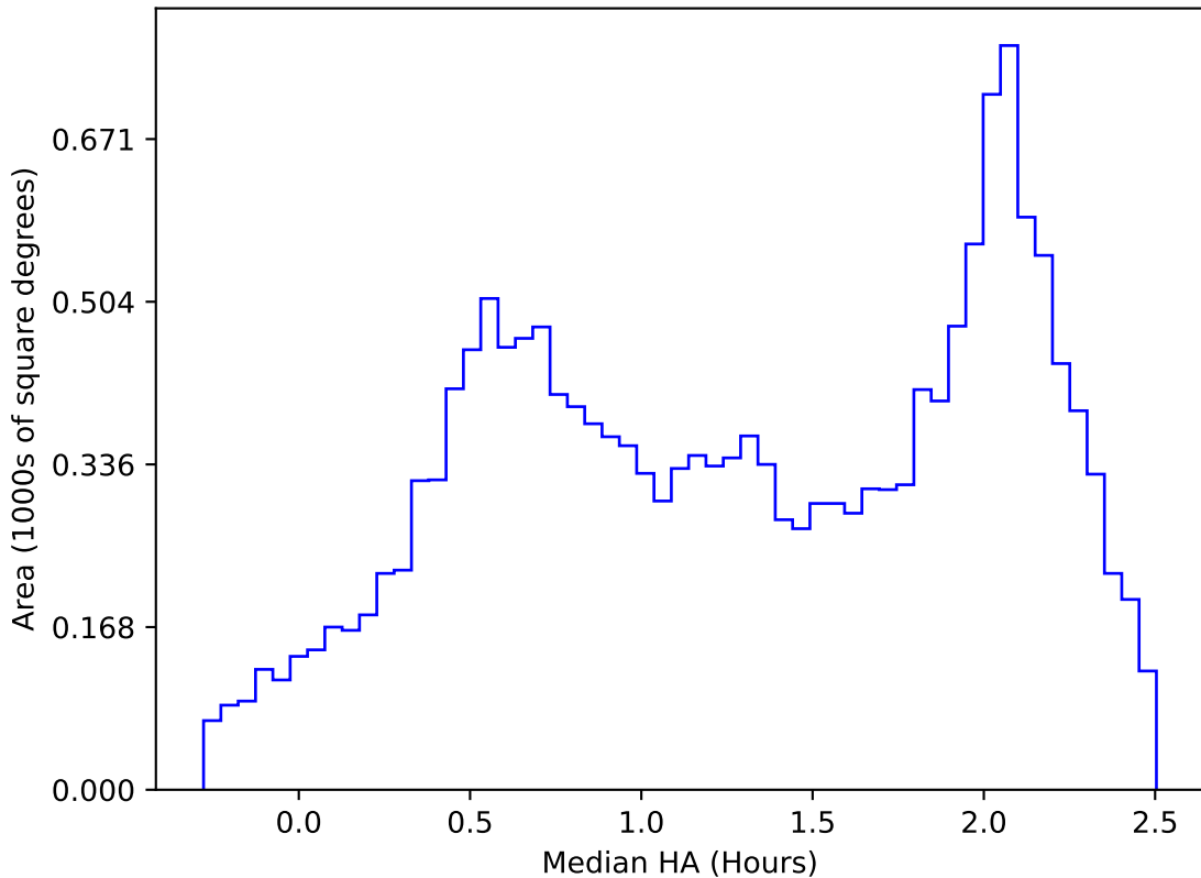
too_elab_r64_d3_giz_v3.4_10yrs WFD y band: Median HA
