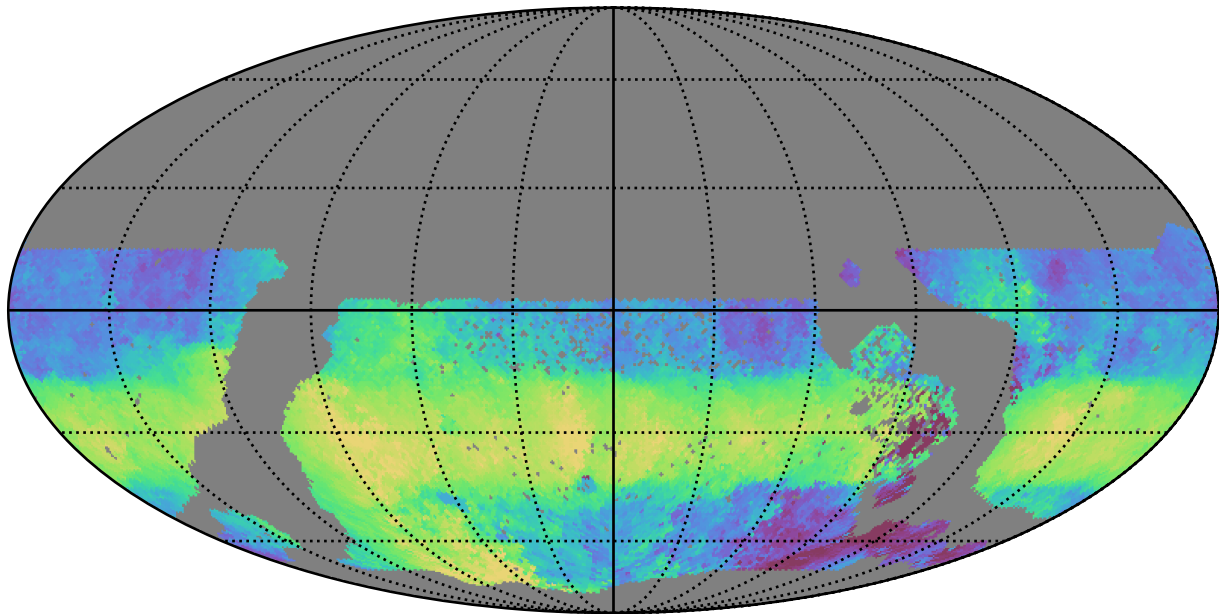
too_elab_r64_d3_giz_v3.4_10yrs WFD u band: Median HA
