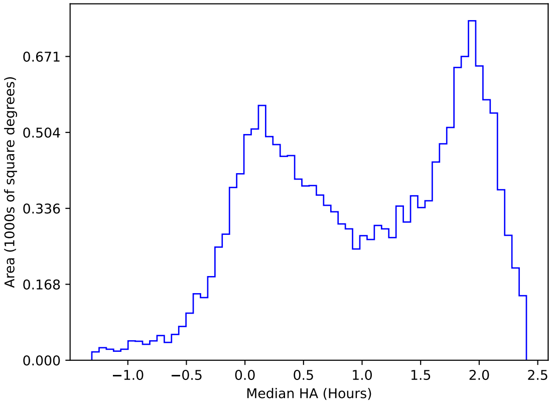
too_elab_r64_d3_giz_v3.4_10yrs WFD u band: Median HA
