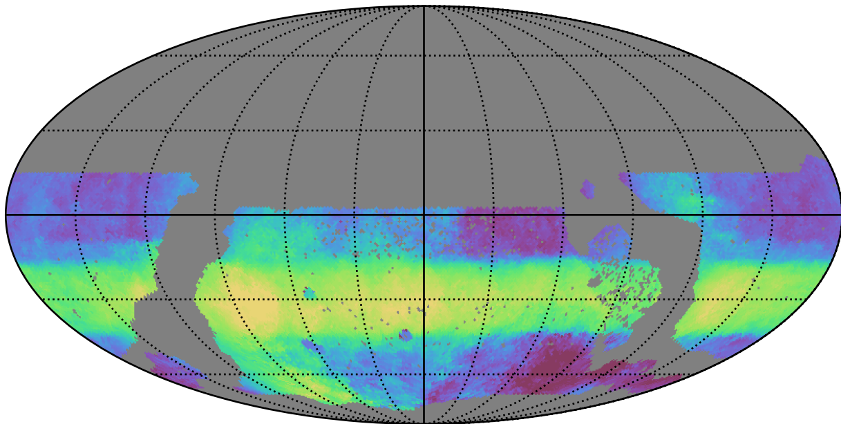
too_elab_r64_d3_giz_v3.4_10yrs WFD r band: Median HA
