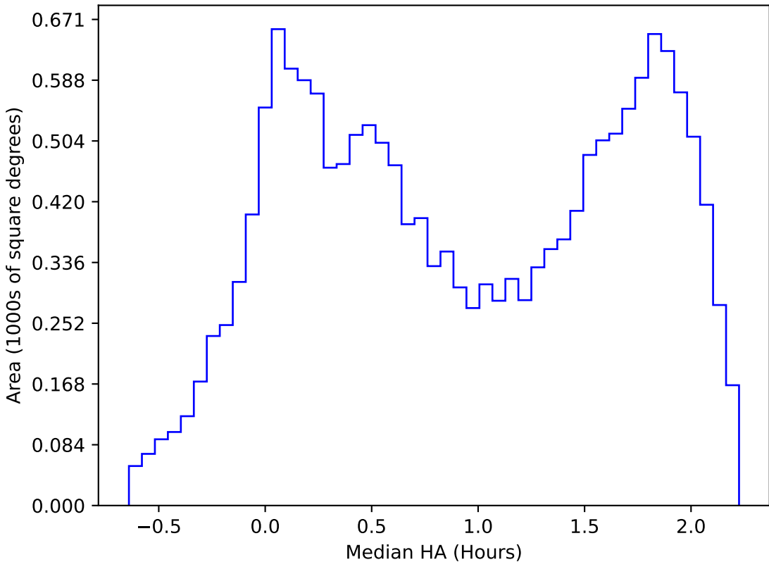
too_elab_r64_d3_giz_v3.4_10yrs WFD r band: Median HA
