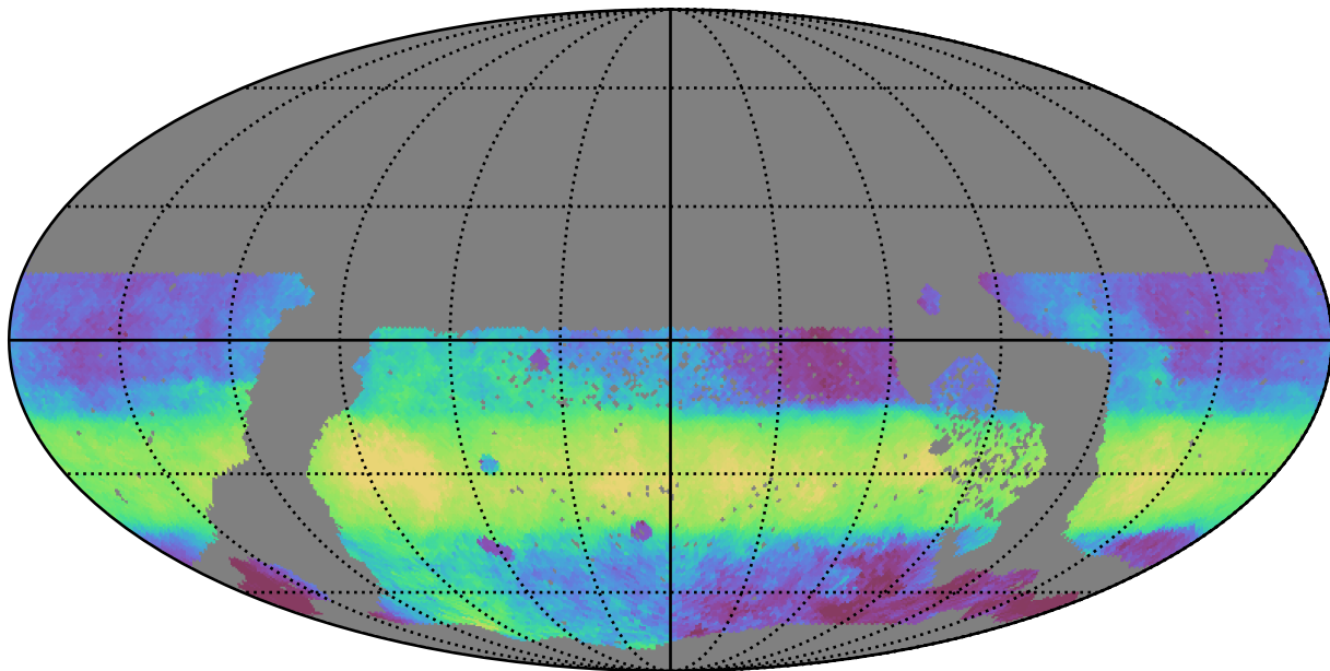
too_elab_r64_d3_giz_v3.4_10yrs WFD i band: Median HA
