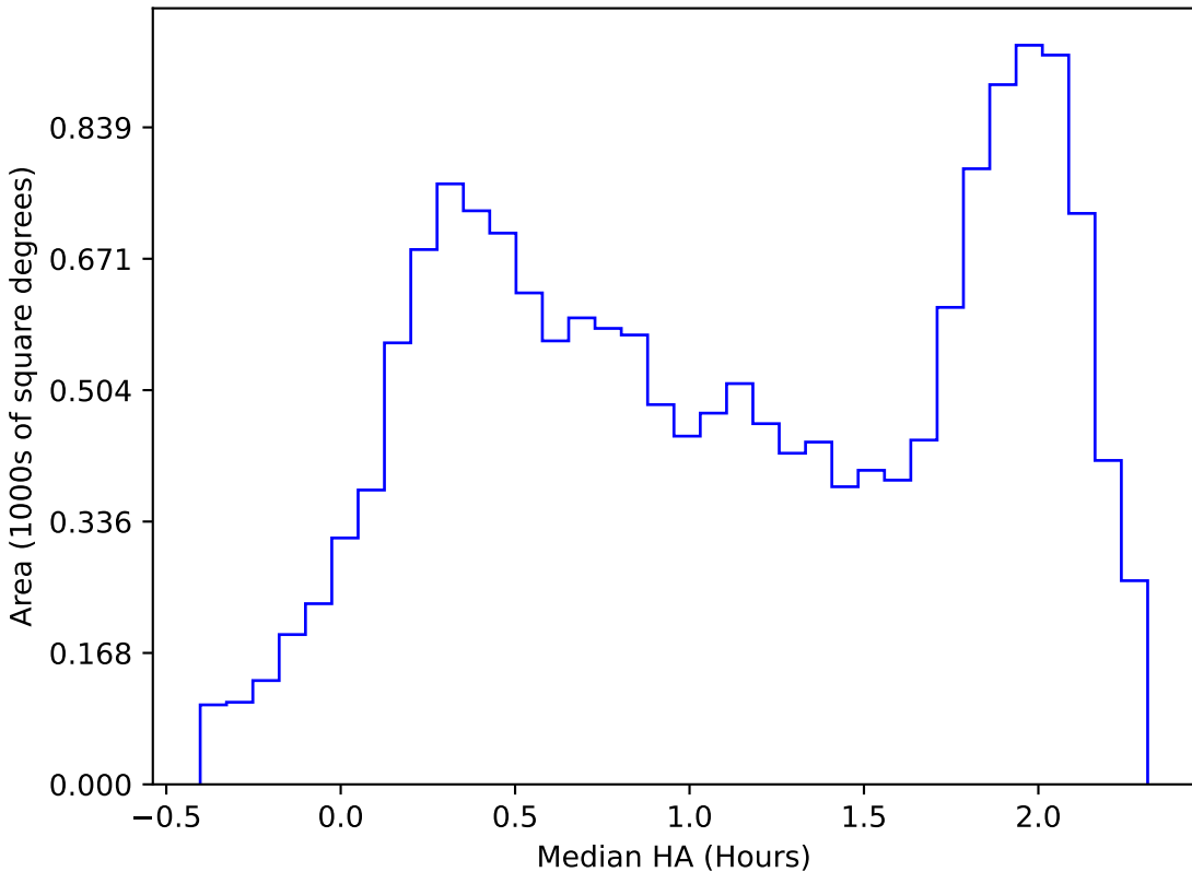
too_elab_r64_d3_giz_v3.4_10yrs WFD i band: Median HA
