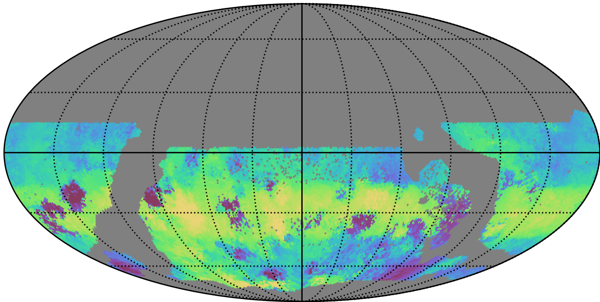
too_elab_r64_d3_giz_v3.4_10yrs WFD g band: Median HA
