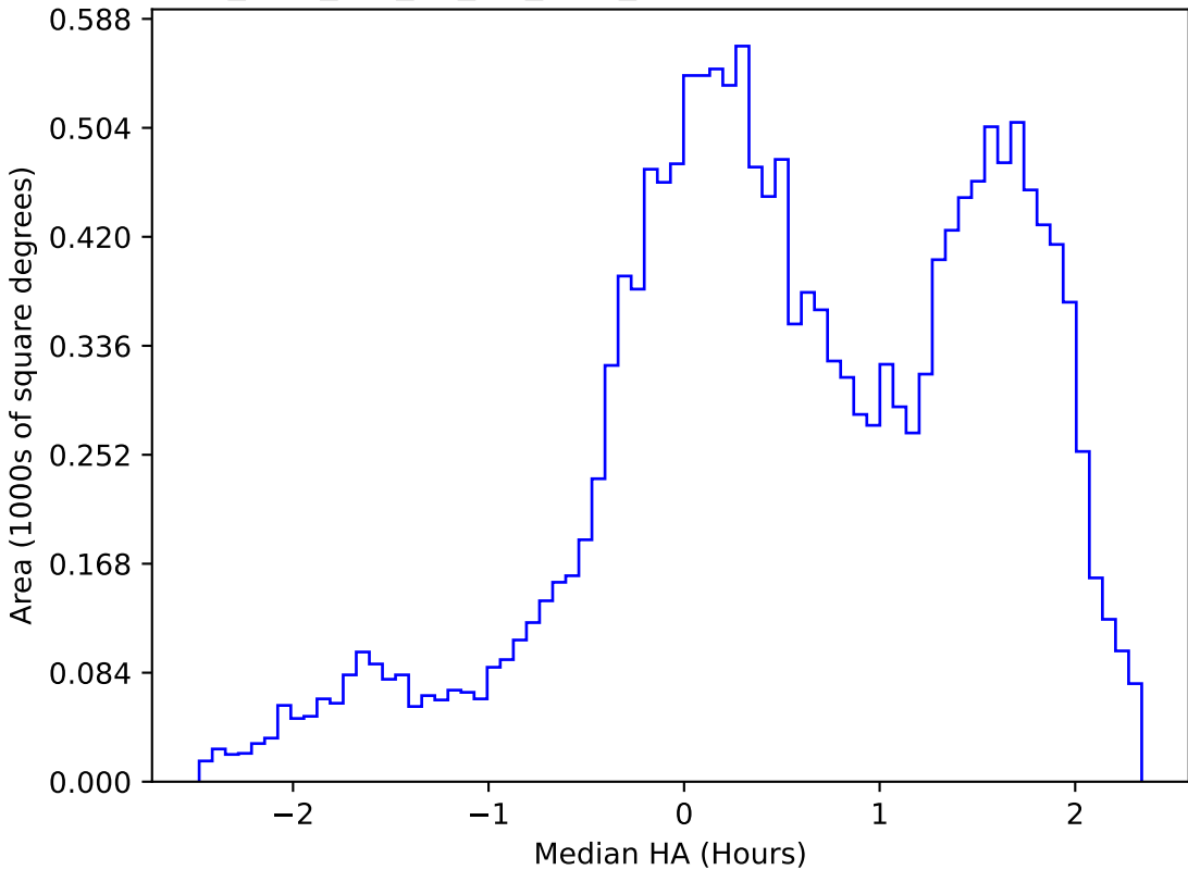
too_elab_r64_d3_giz_v3.4_10yrs WFD g band: Median HA
