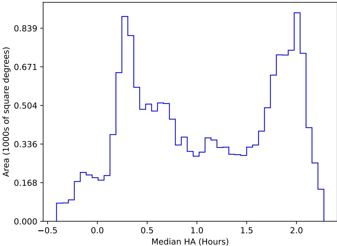
too_elab_r64_d3_giz_v3.4_10yrs WFD all bands: Median HA
